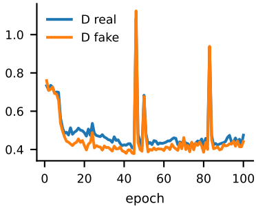
Discriminator losses
