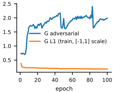
Generator losses
