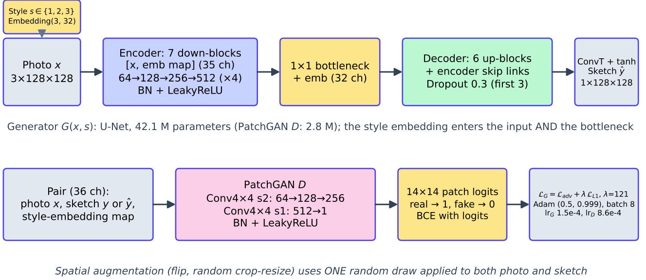
Task 4 - style-conditioned pix2pix-style cGAN
