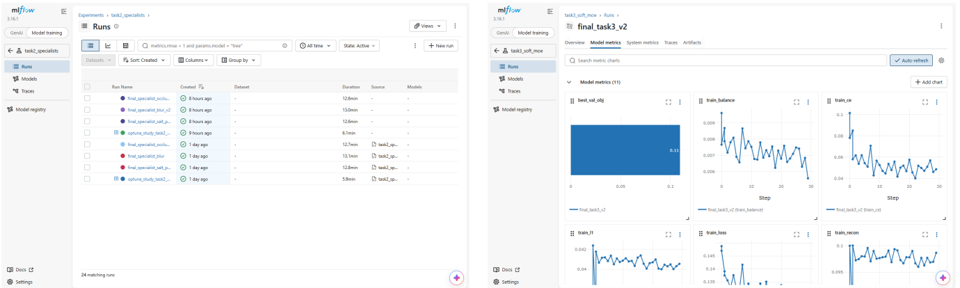
Fig. 27. MLflow interface: the experiments with their runs (left) and the metrics of one training run (right).
