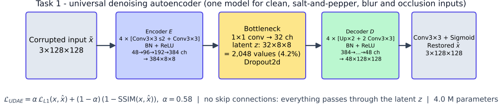
Fig. 2. Universal denoising autoencoder: the only path from input to output is the 2,048-value latent.
