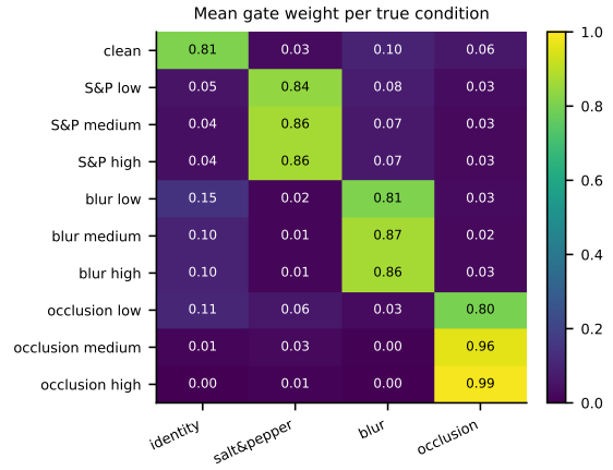
Fig. 13. Routing heat-map: mean weight of each branch by true corruption and severity.
