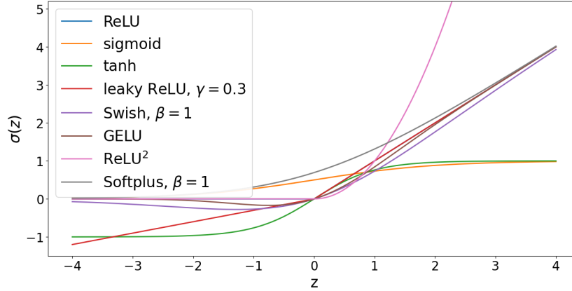
Figure 7.3: Activation functions in deep learning. The y-axis is capped above 5 for visualization.
