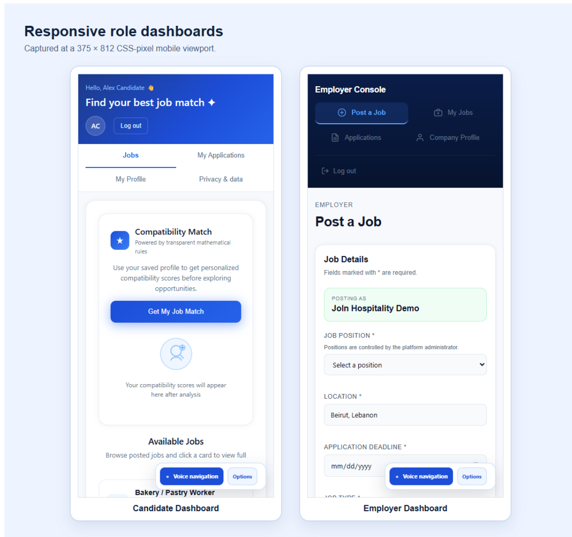
Figure 16: Responsive role dashboards
