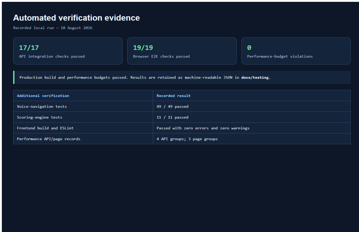
Figure 17: Integration, E2E, and performance evidence
