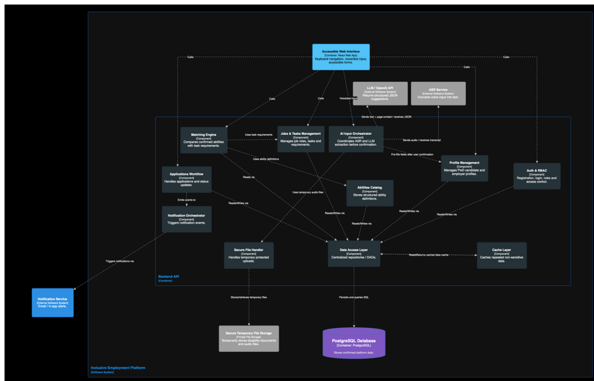
Figure 10: Component diagram
