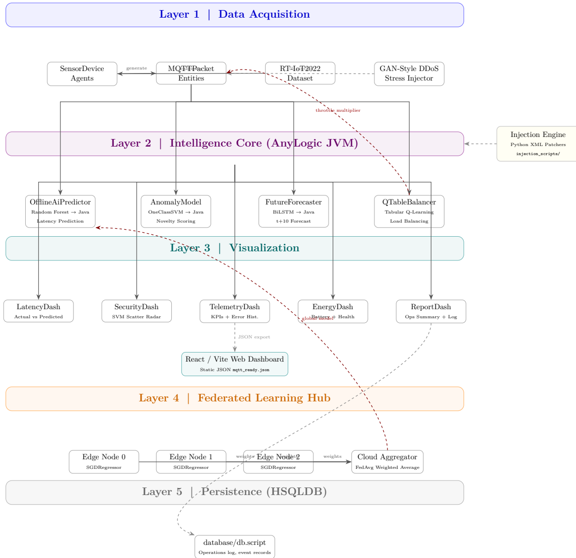
Figure 3.1: Complete Aegis-IoT system architecture: five layers from data acquisition through intelligence, visualization, federated learning, and persistence. Dashed arrows indicate asynchronous or offline data paths; red dashed arrows indicate feedback loops.
