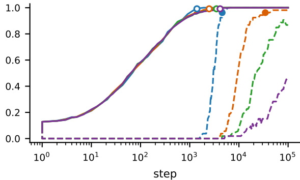
accuracy
