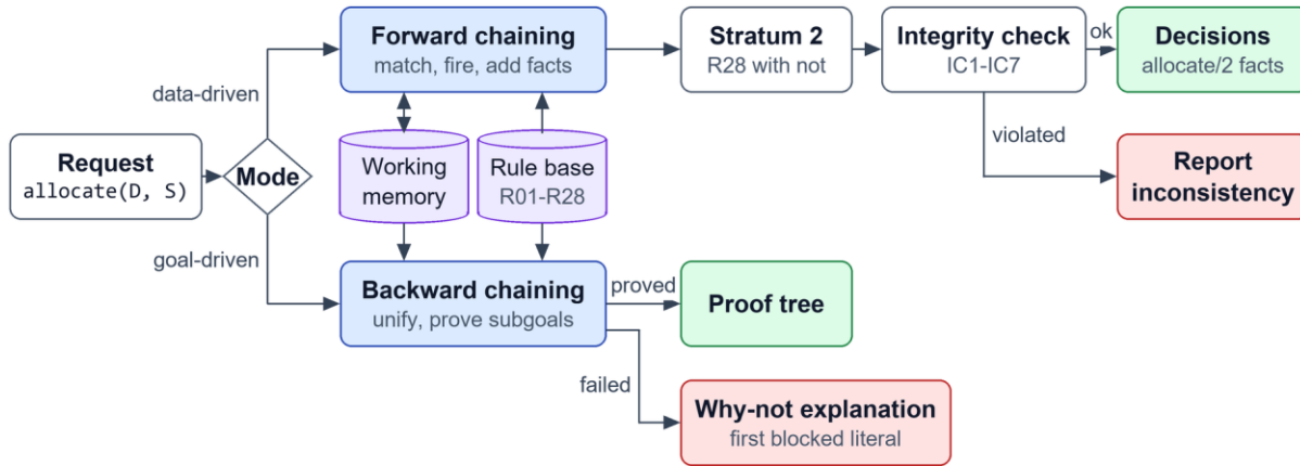
Figure 6: Inference engine architecture
