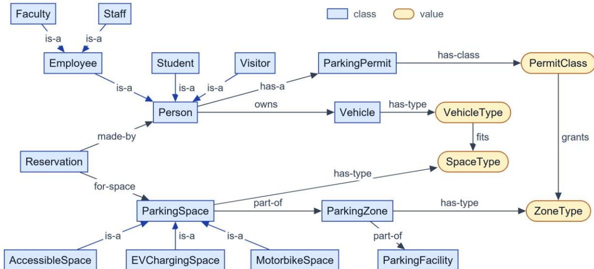
Figure 4: Concept-level semantic network
