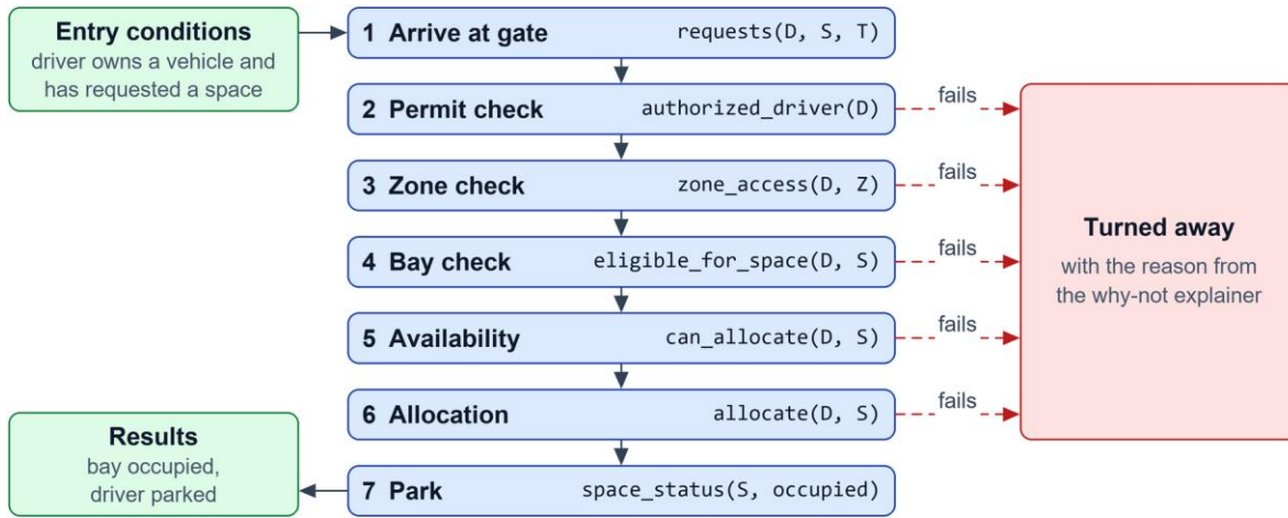
Figure 3: ParkingSession script scenes
