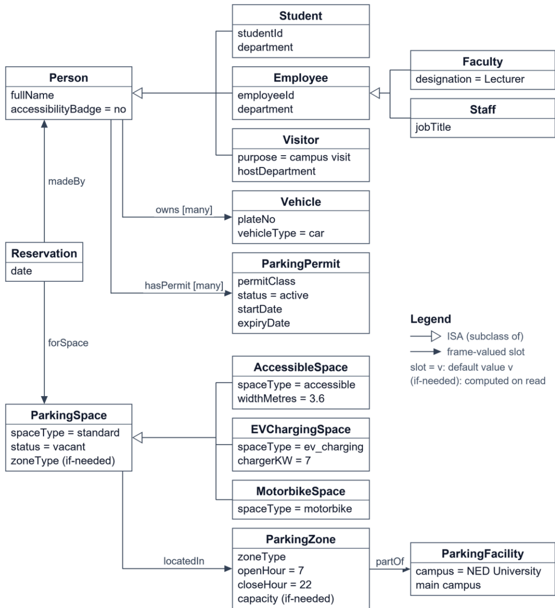
Figure 2: Frame hierarchy with slots and links
