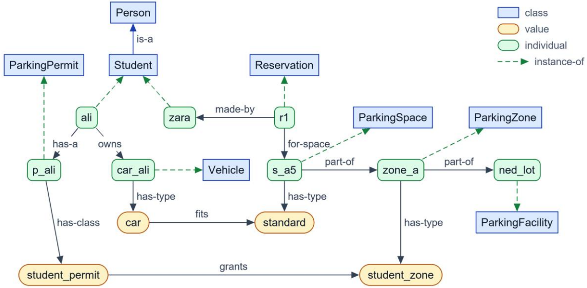
Figure 5: Semantic network with individuals
