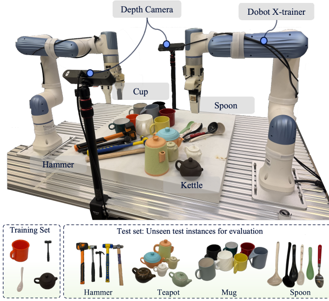
Fig. 3: Real-world experimental setup on the DOBOT X-Trainer dual-arm platform. The bottom row shows the object instances used for training and the geometrically and visually different held-out instances used for evaluation.
