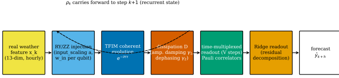
Figure 1: Sequential dissipative reservoir pipeline. \rho_k (dashed feedback) carries the recurrent quantum state from step k to k+1 – the architectural feature Sec. 6.1’s central ablation isolates.
