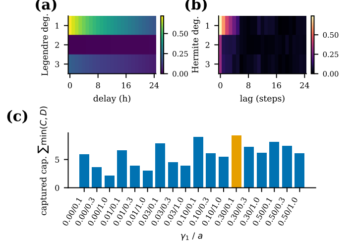
Figure 2: (a) Task demand D(\text{delay}, \text{degree}) at h=6 . (b) Reservoir supply C(\text{lag}, \text{degree}) at the matched configuration. (c) Captured capacity \sum \min(C, D) across the (\gamma_1, a) grid; the matched configuration (highlighted) is the grid maximum.
