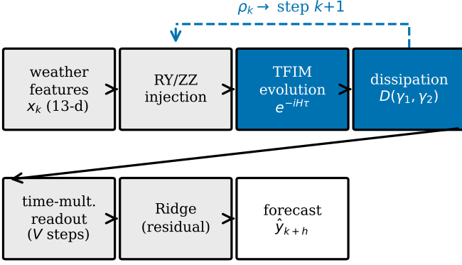
Figure 1: Sequential dissipative reservoir pipeline. \rho_k (dashed feedback) carries the recurrent quantum state from step k to k+1 – the architectural feature Sec. 6.1’s central ablation isolates.
