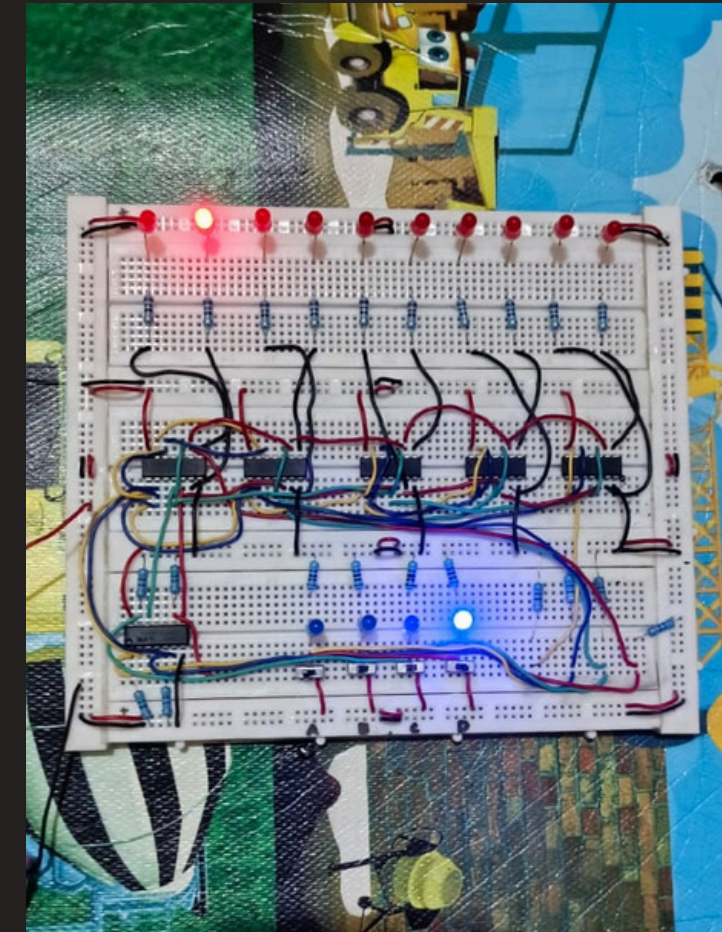
Logic Circuit Design Decoder 10 Output
