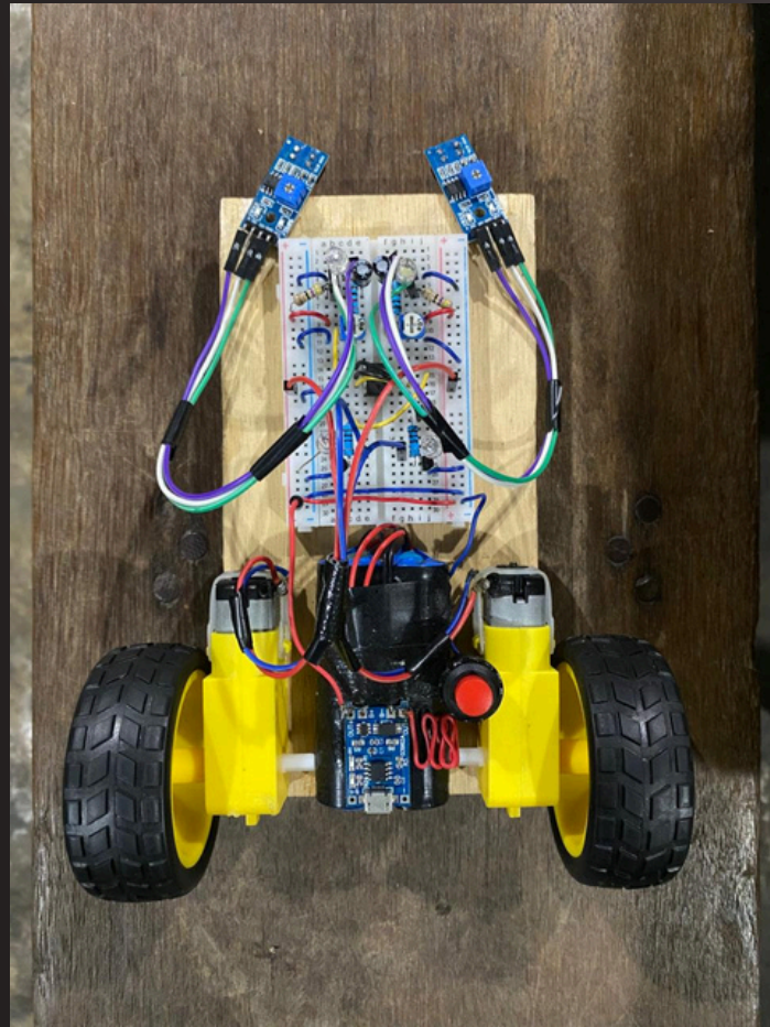
Line Follower Analog
