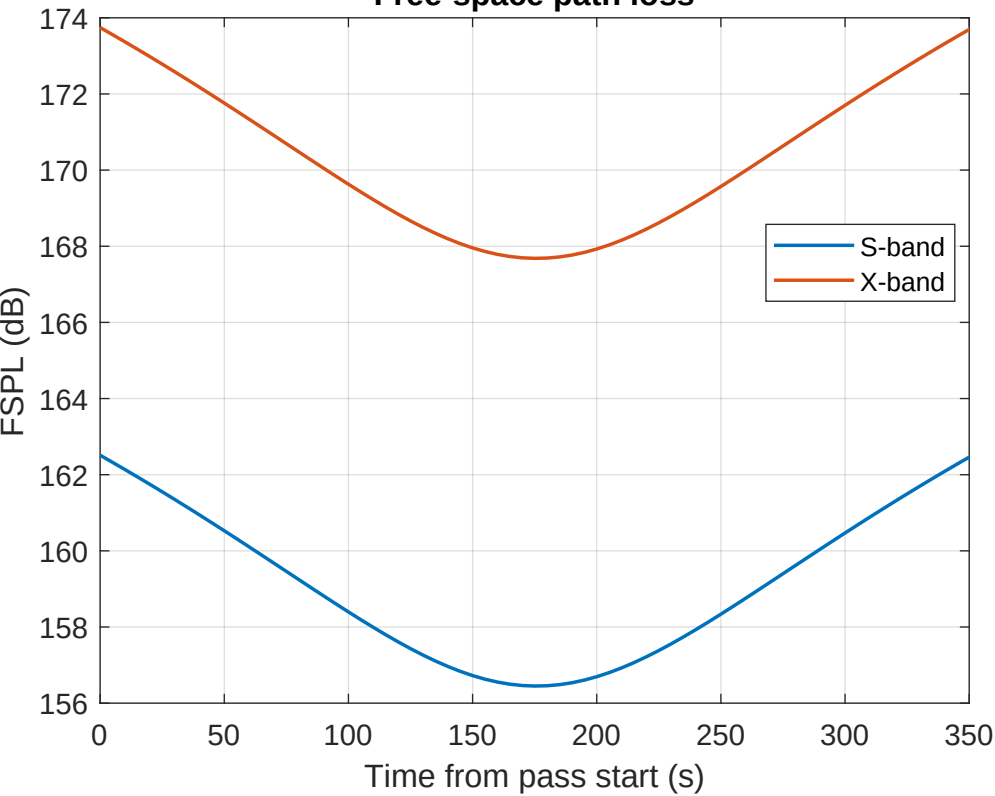
Free-space path loss
