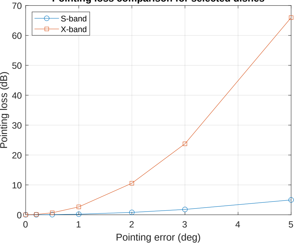
Pointing loss comparison for selected dishes
