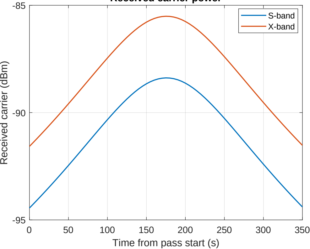
Received carrier power
