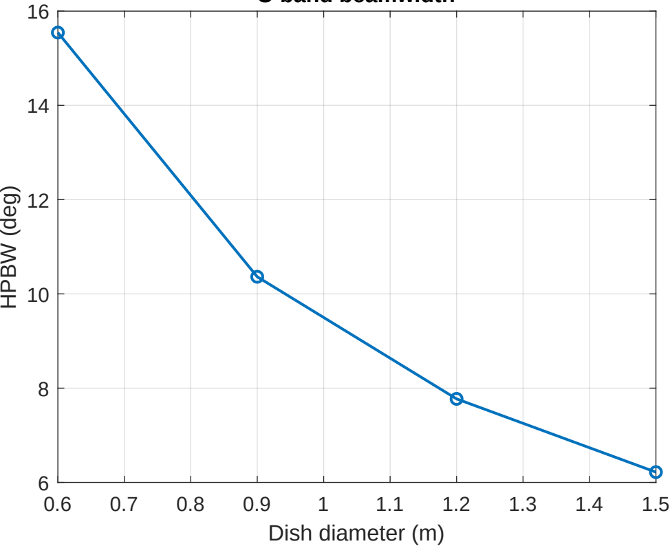
S-band beamwidth
