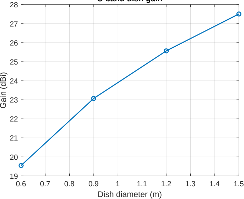
S-band dish gain
