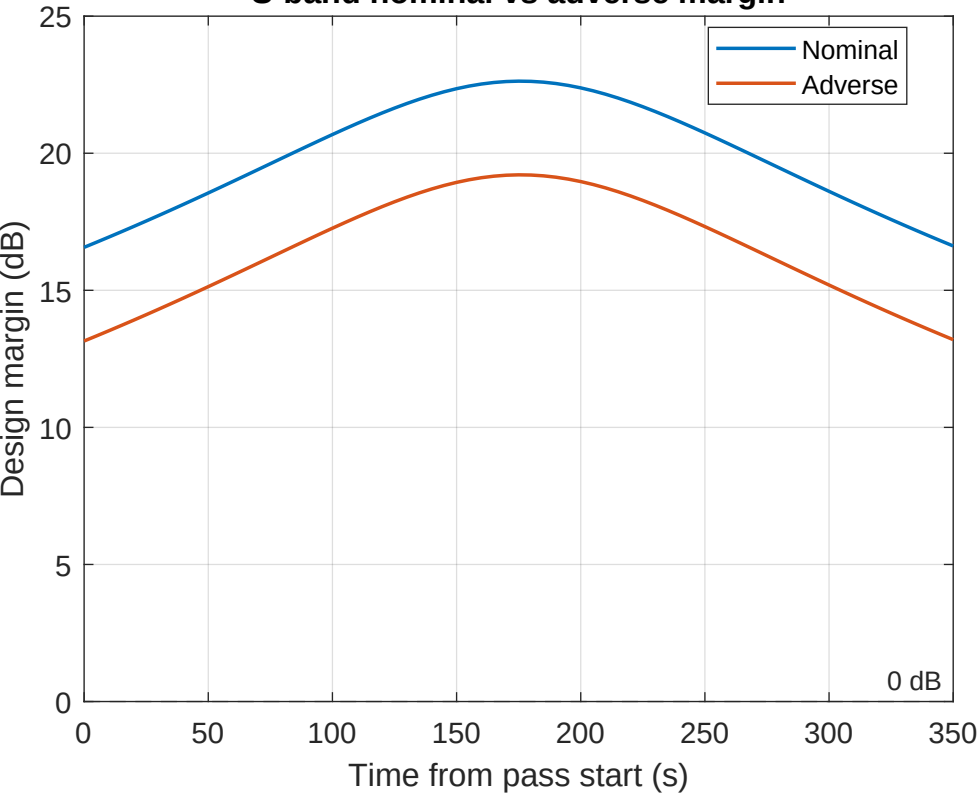
S-band nominal vs adverse margin
