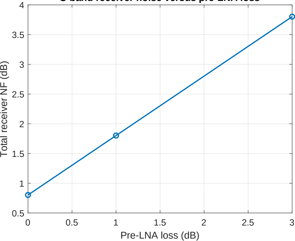
S-band receiver noise versus pre-LNA loss
