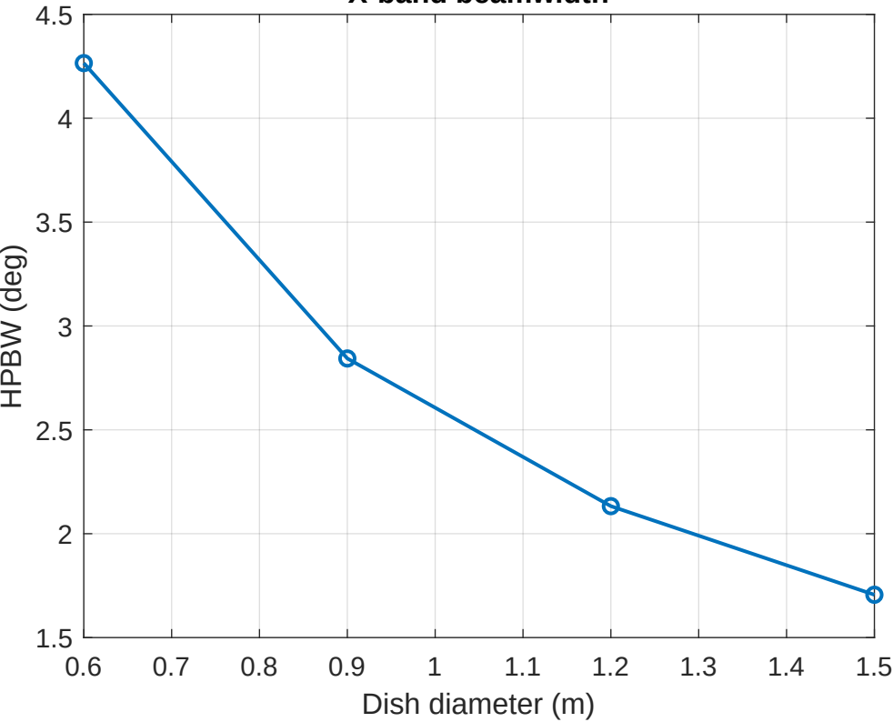
X-band beamwidth
