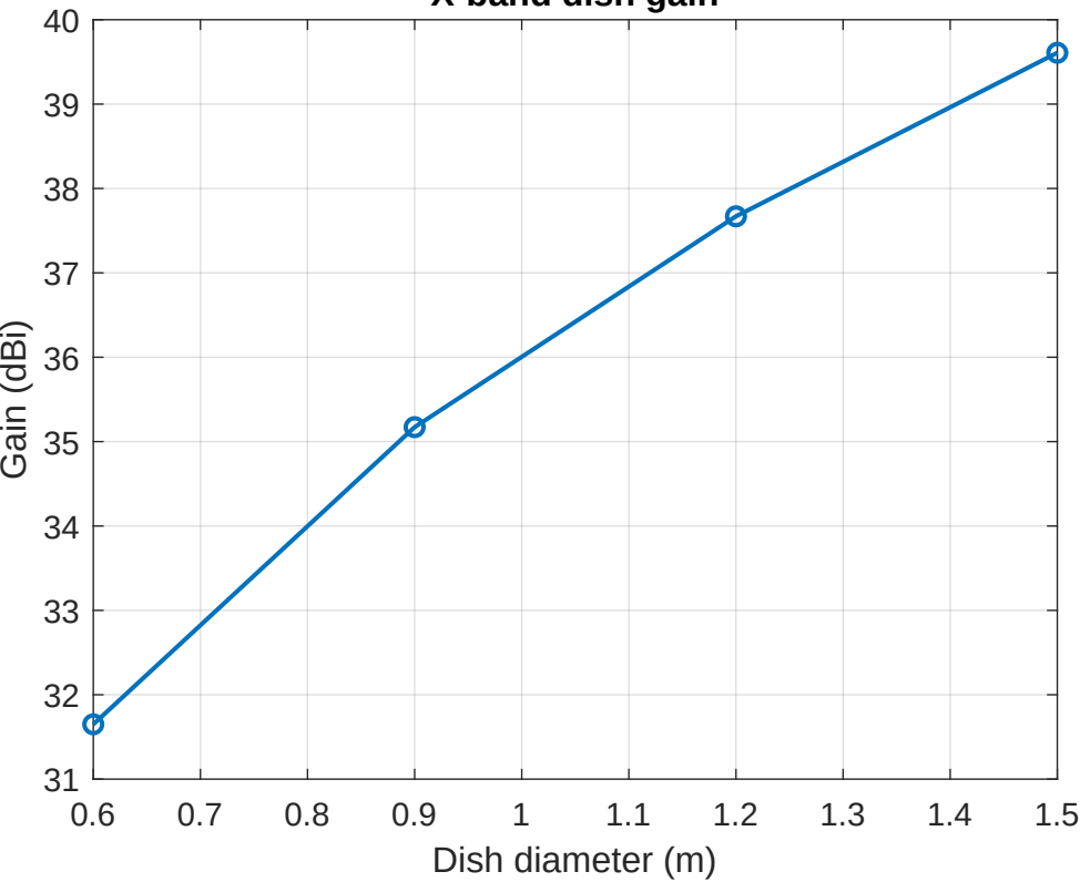
X-band dish gain
