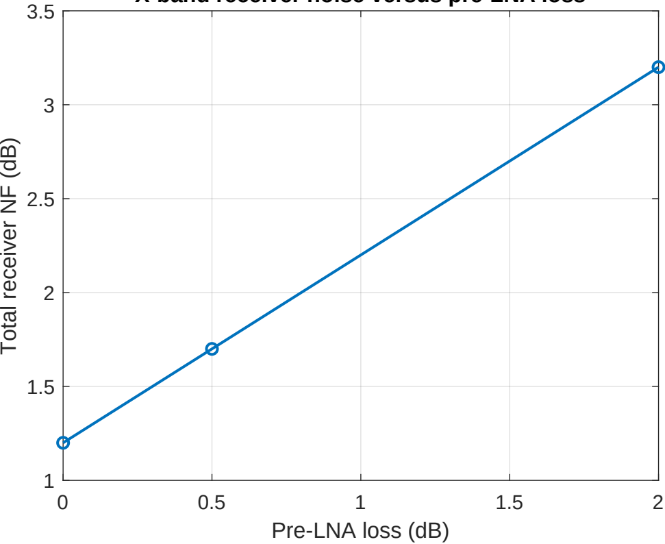
X-band receiver noise versus pre-LNA loss
