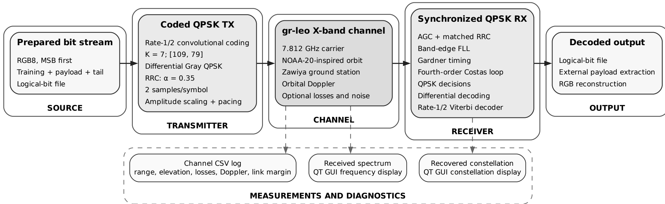
High-level architecture of the GNU Radio image-transmission and LEO downlink simulation.
