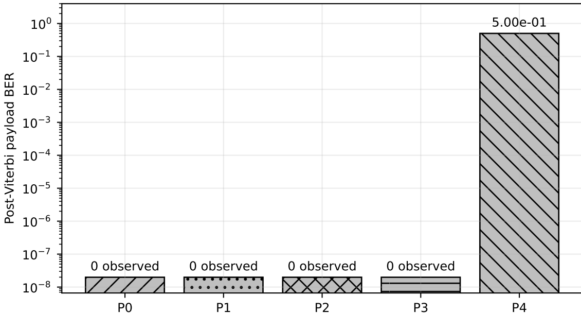
BER by fixed channel profile
