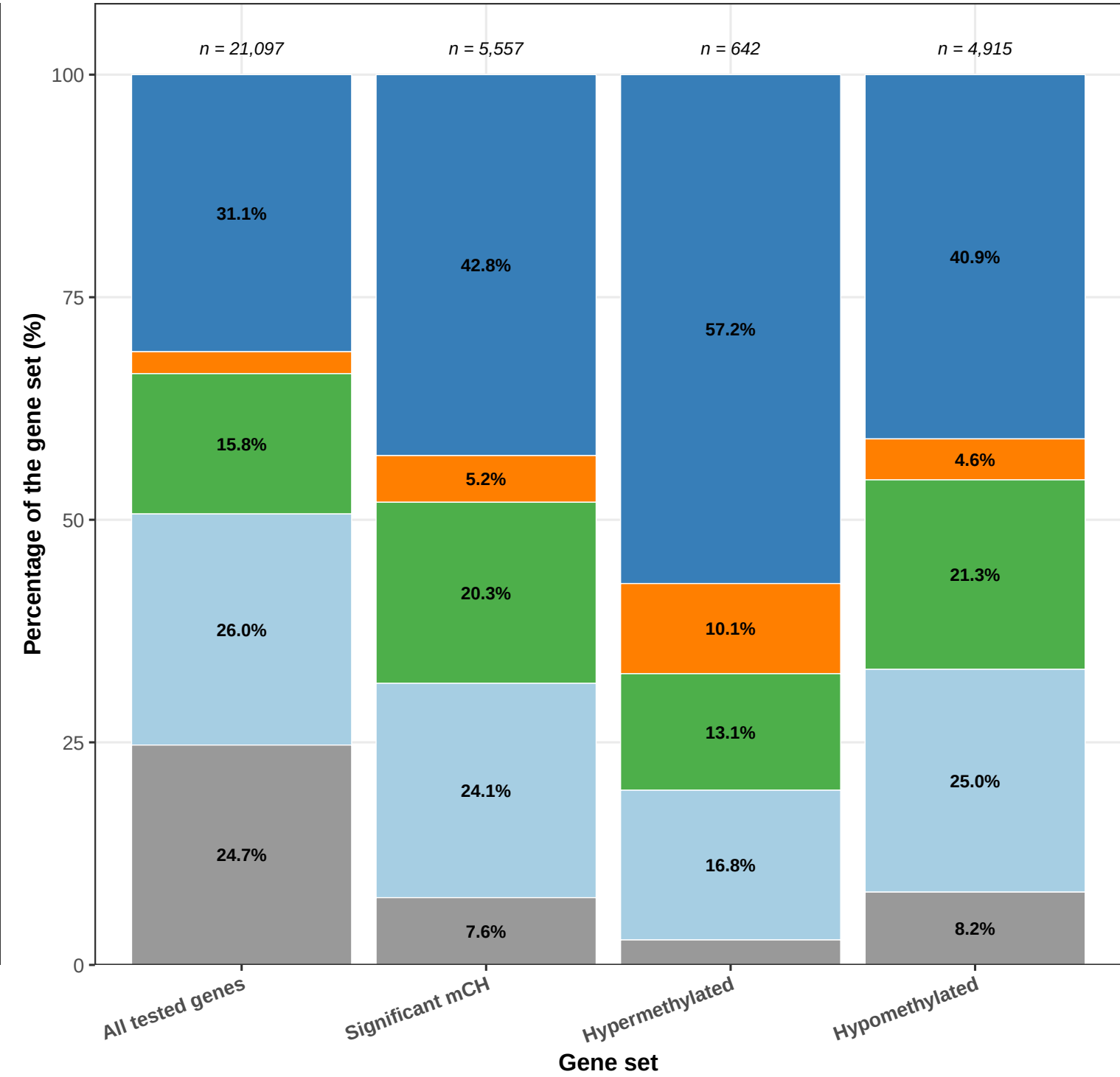
Gene-body state
