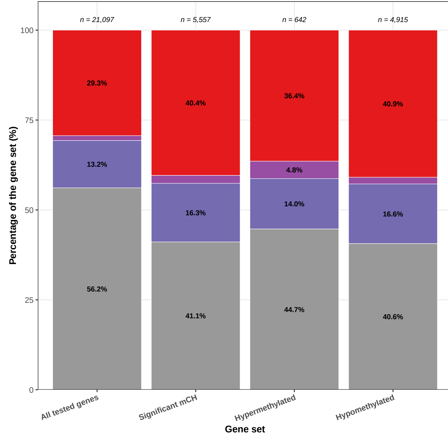
Promoter state
