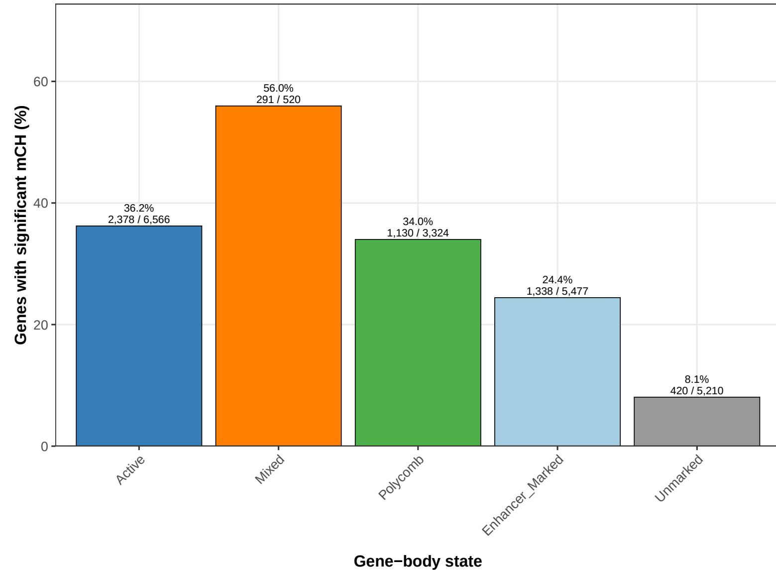
Gene-body state
