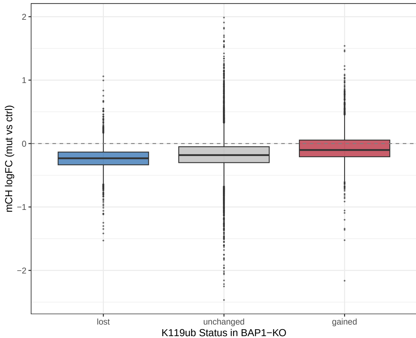
mCH Change by K119ub Direction
