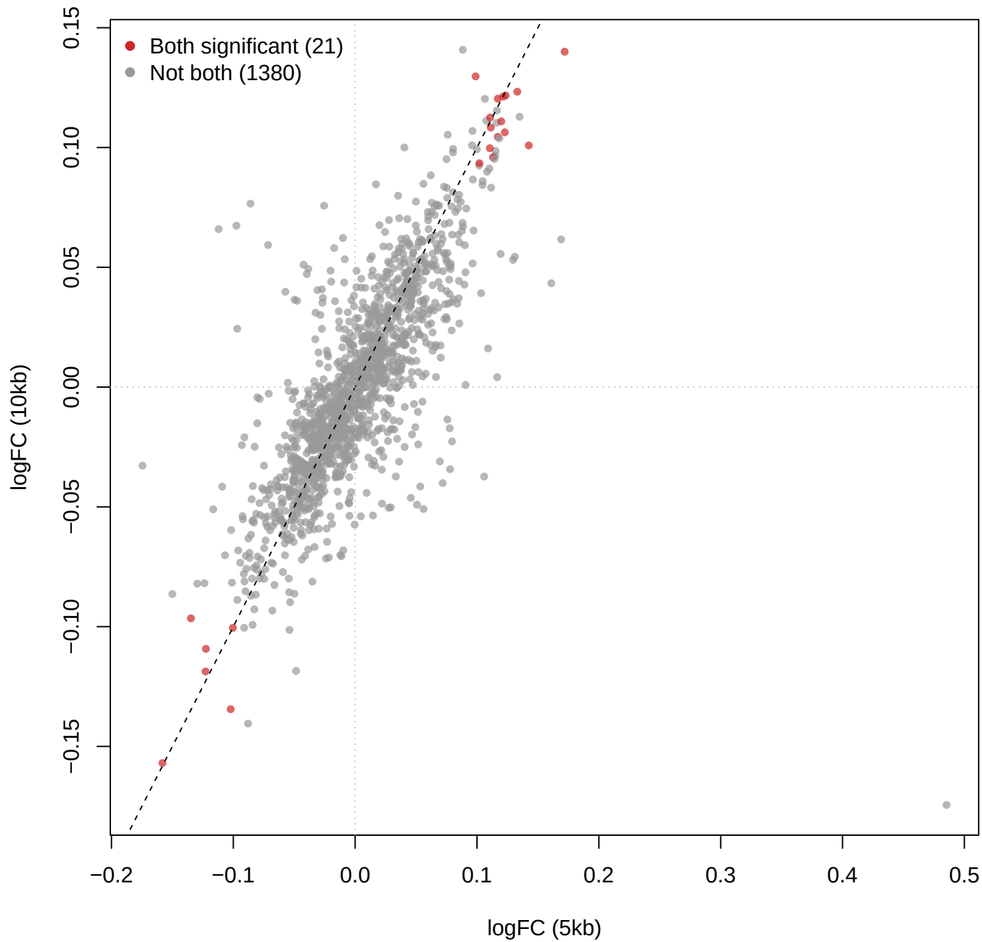
logFC Correlation (250831) r = 0.738 , n = 1401 matched
