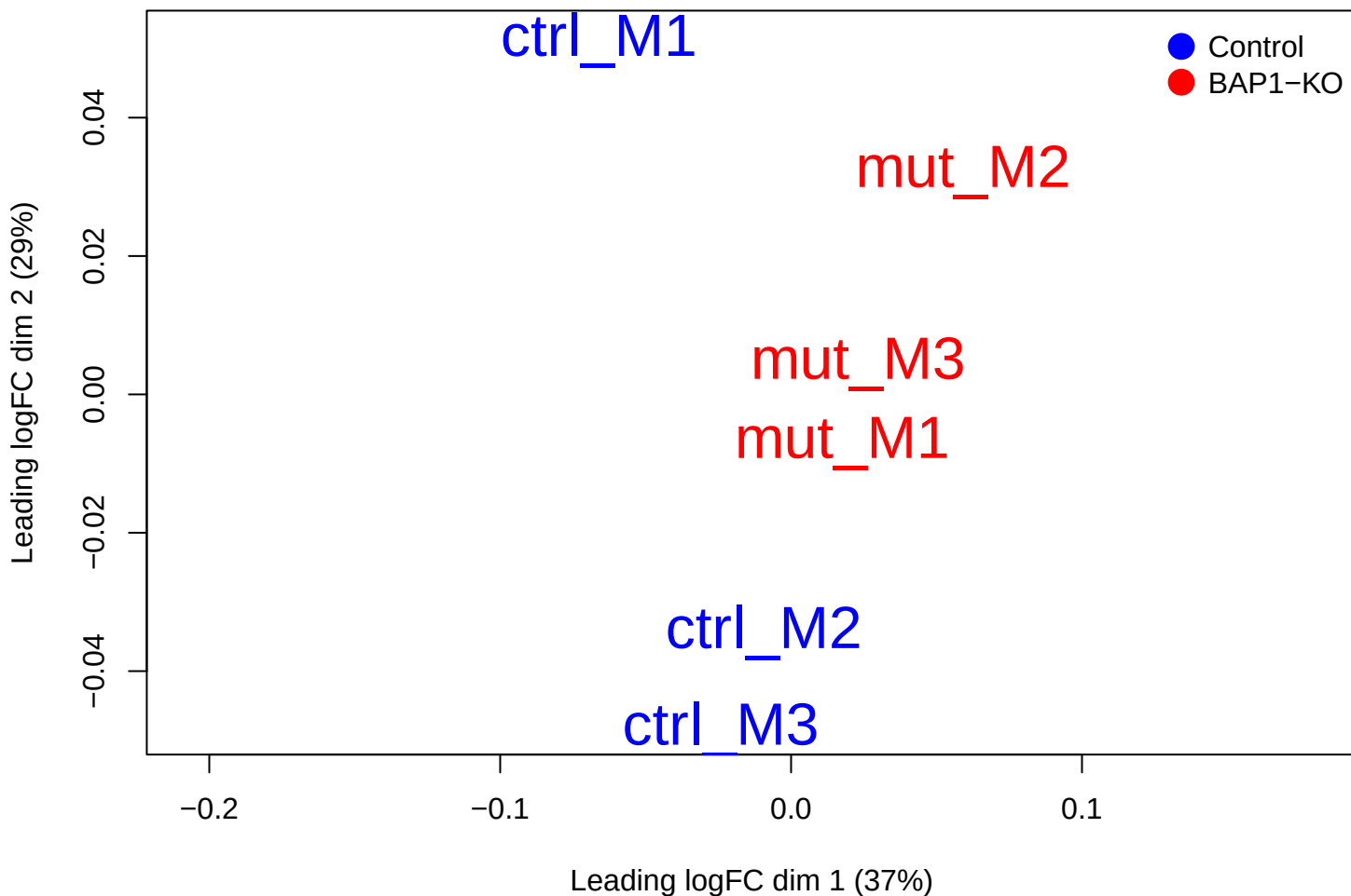
MDS Plot – Stripenn Stripes (250831, 10kb)
