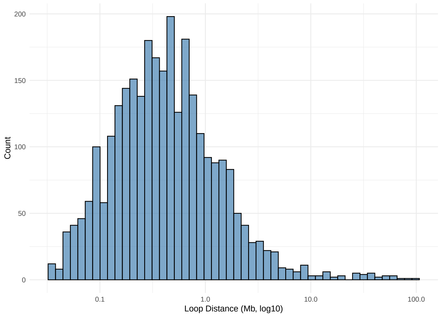
Distribution of Loop Distances
