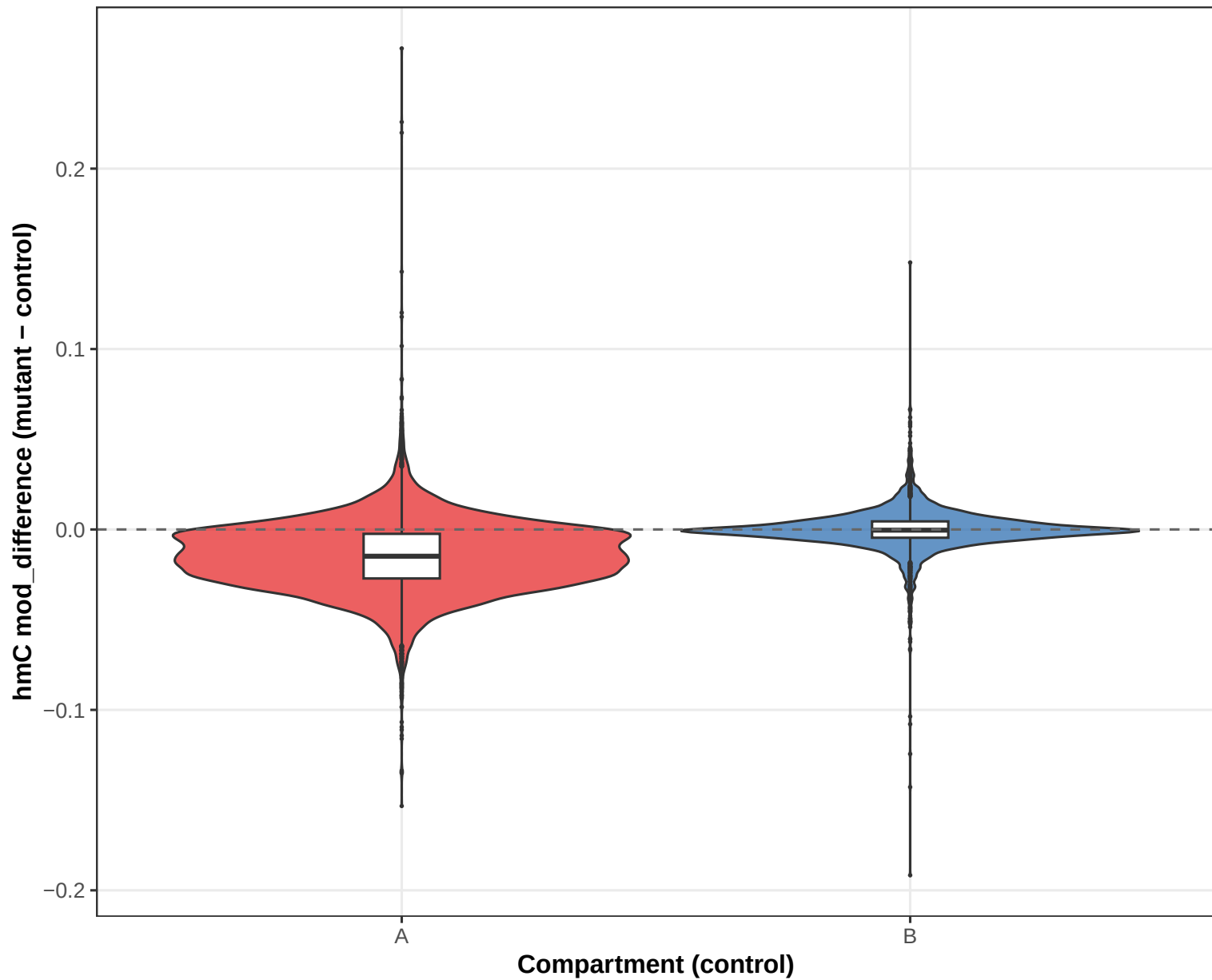
5hmC Change by A/B Compartment Wilcoxon p < 2.2e-16 | A: n=12347, B: n=3739
