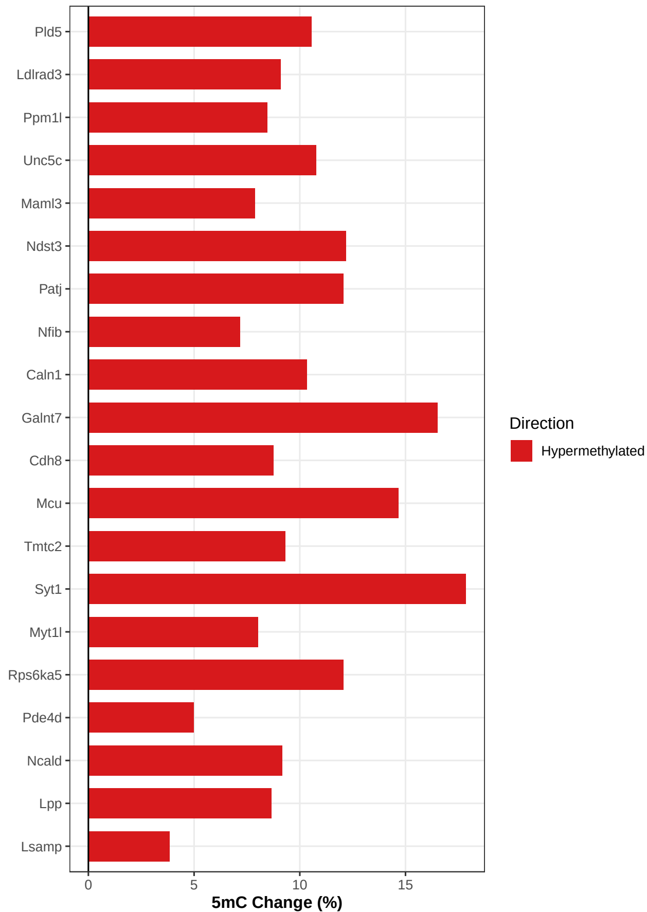
Top 20 Gene Body 5mC DMRs Ranked by q-value | BAP1-KO vs Control
