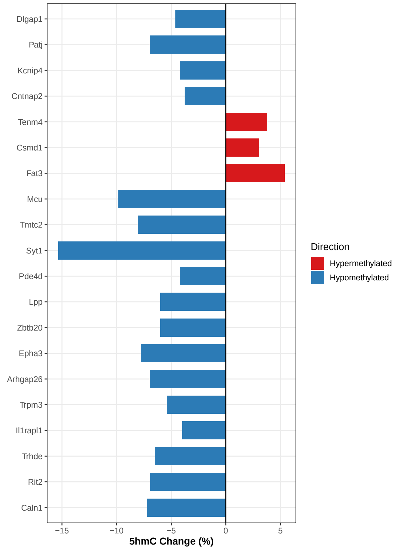
Top 20 Gene Body 5hmC DMRs Ranked by q-value | BAP1-KO vs Control
