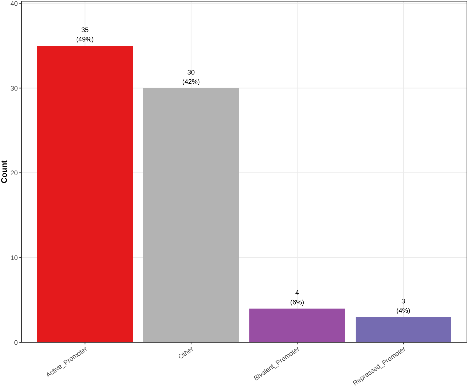
Chromatin states of MeCP2-Up + K119ub-Up genes (n=72)
