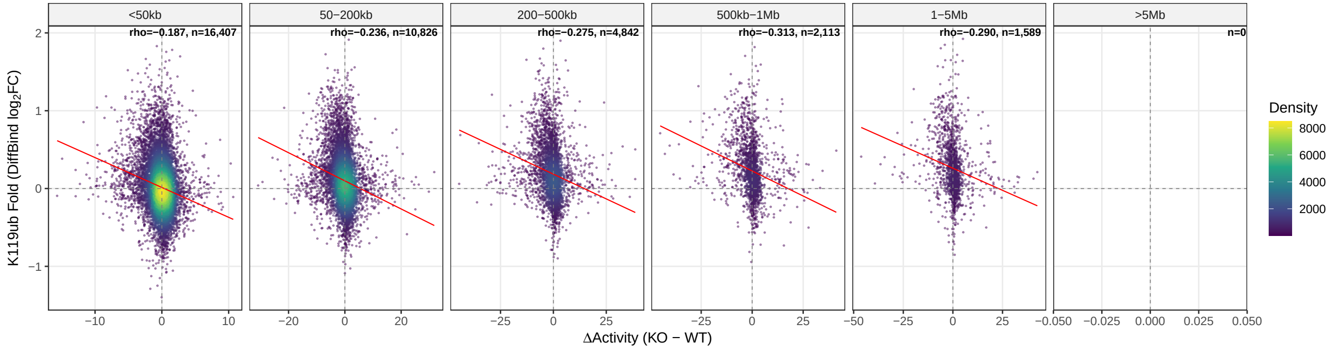
Activity-K119ub correlation by enhancer-gene distance
