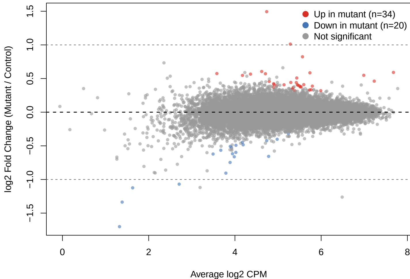
MA Plot (BCV = )
