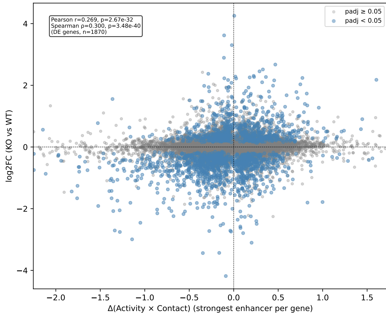
Unnormalized Score
