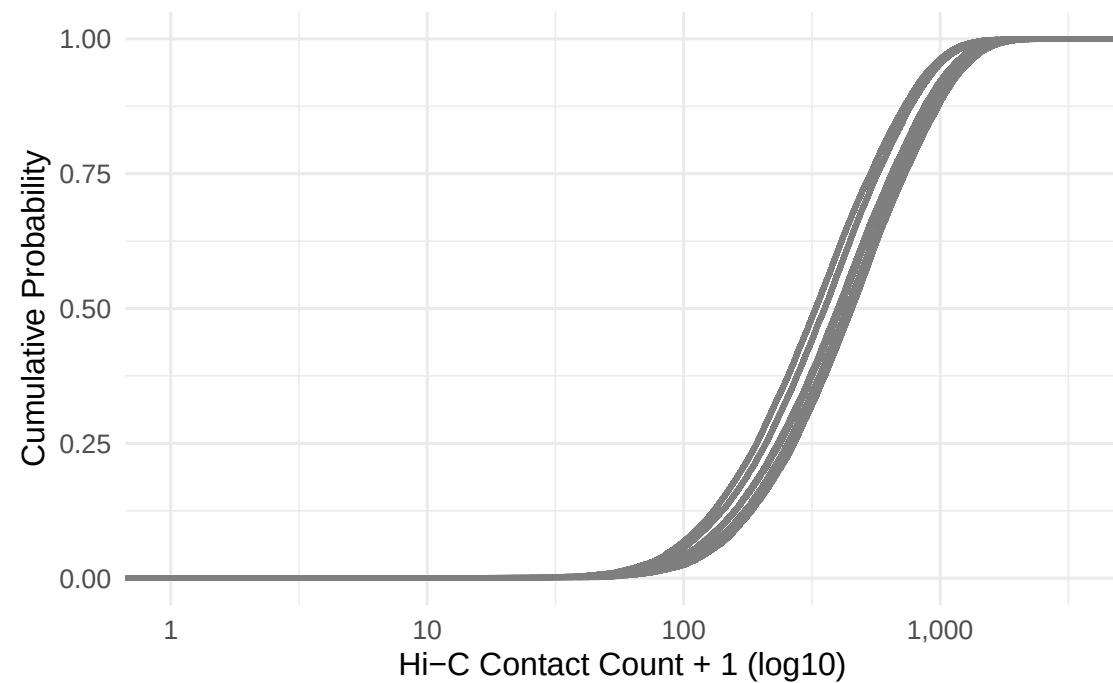
Cumulative Distribution
