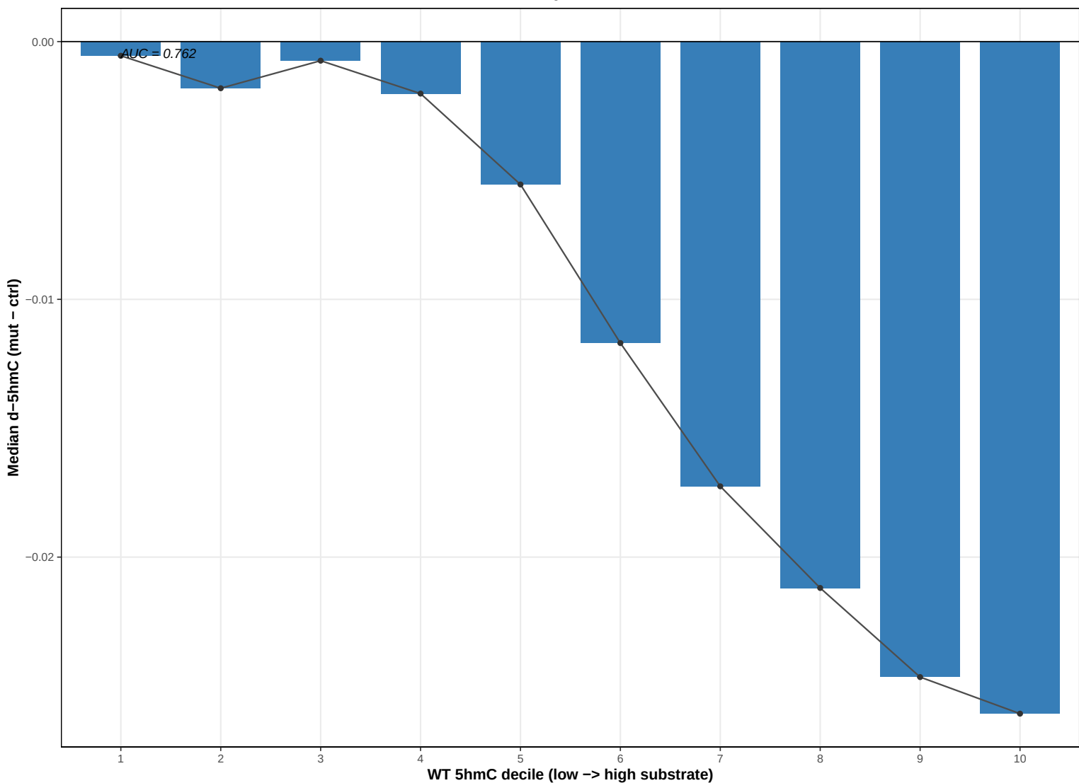
Baseline 5hmC predicts 5hmC loss
