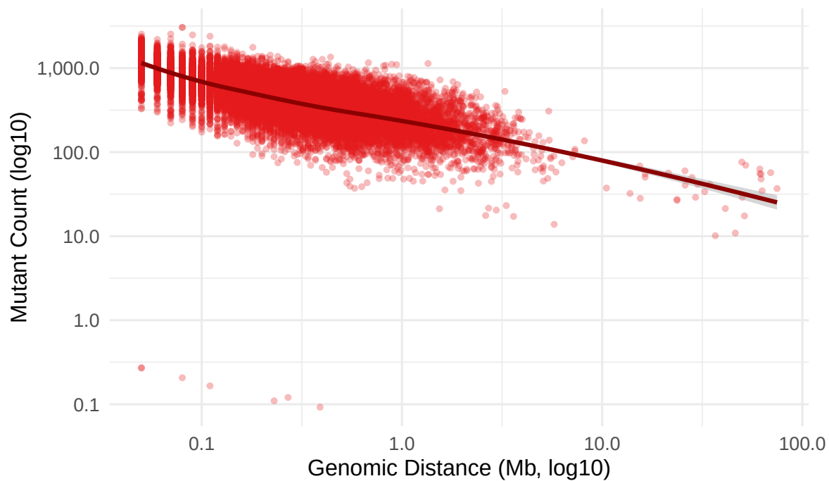
Distance Decay: Mutant
