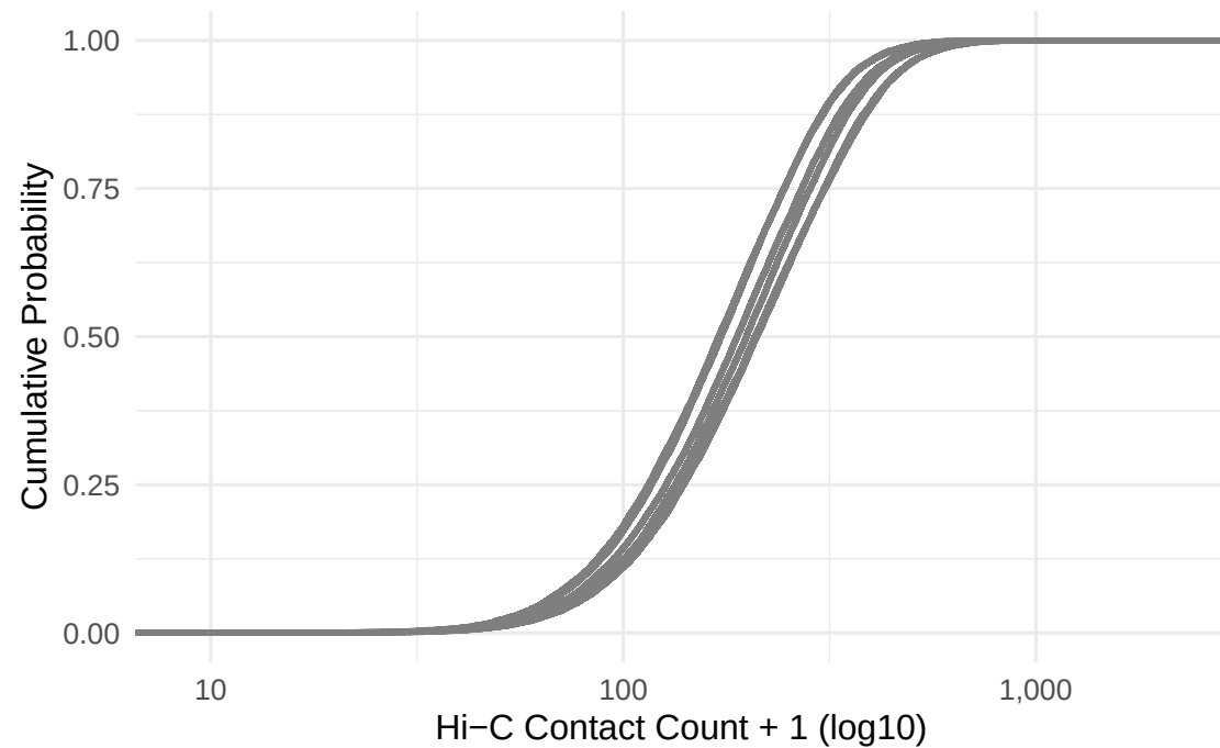
Cumulative Distribution
