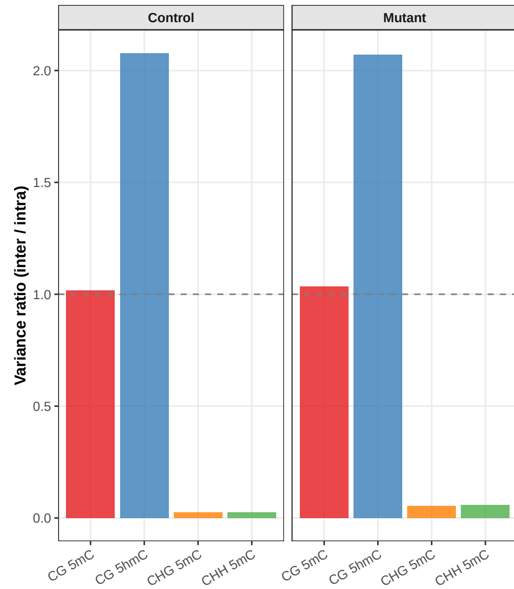
C. Variance Ratio
