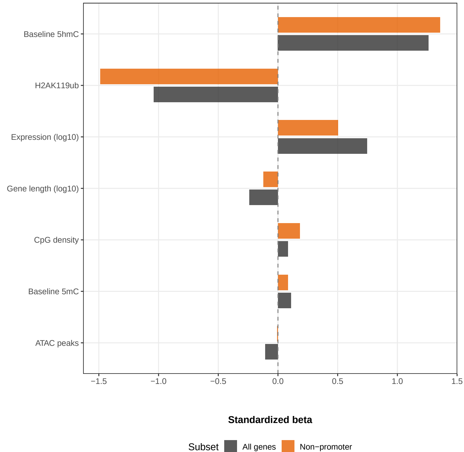
Standardized Betas (Full Model)
