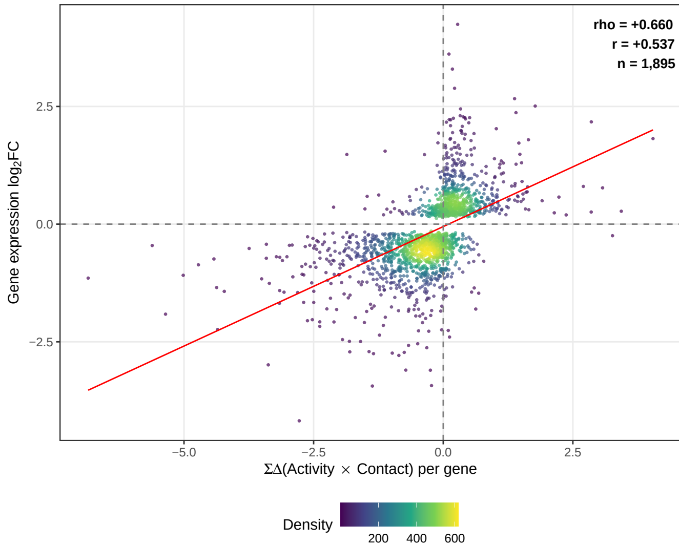
Combined \Delta(A \times C) vs gene expression (baseline)
