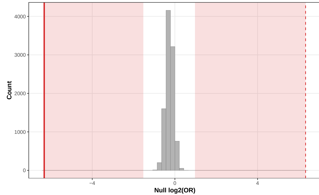
37-07d (z=28.8, p=0.000) mC direction x K119ub DiffBind
