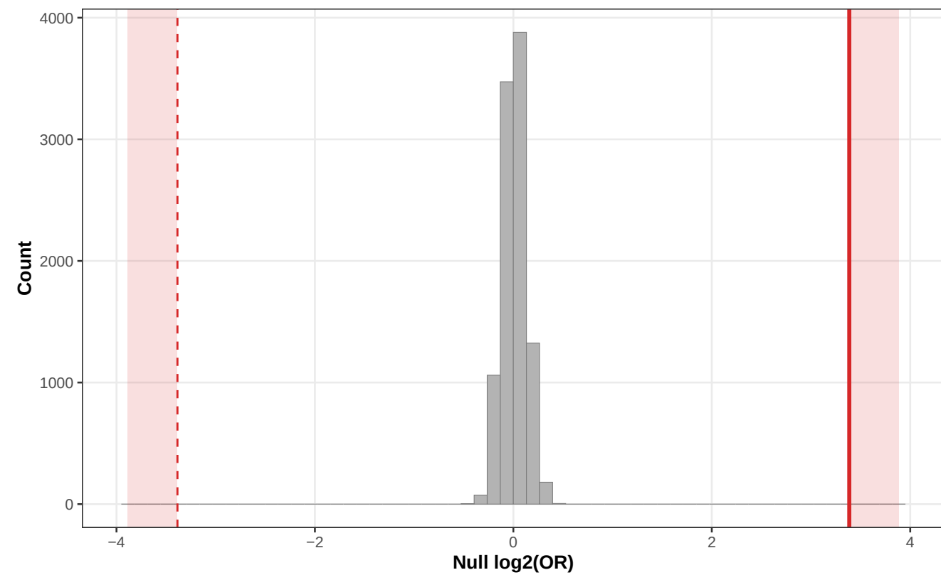
37-03 (z=28.7, p=0.000) hmC direction x ATAC direction
