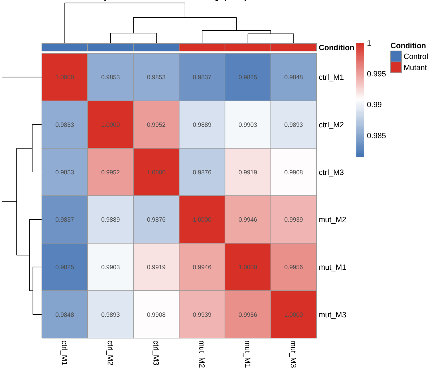
Replicate Correlation: Early (P12) 5kb
