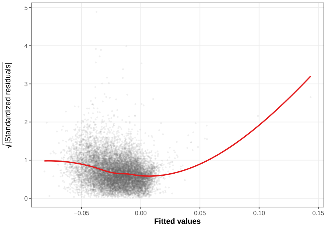
Scale-Location
