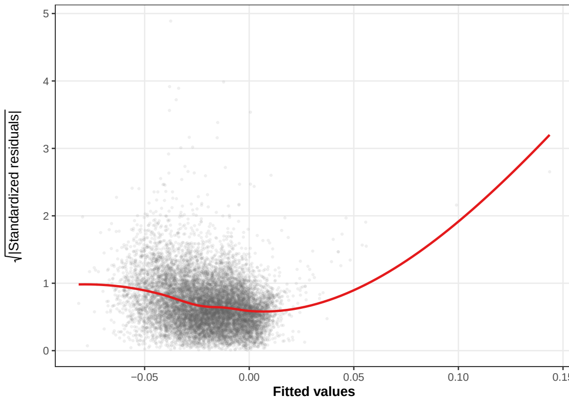
Scale-Location
