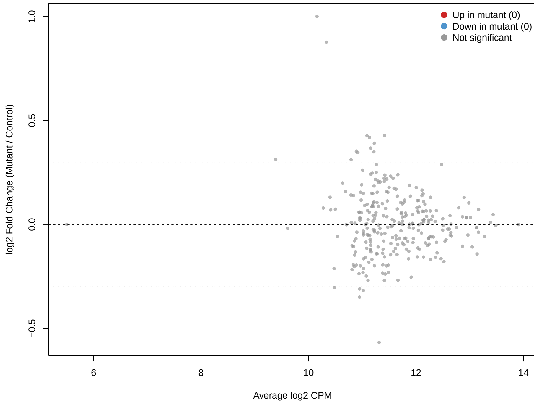
MA Plot – Differential Stripes (early)
