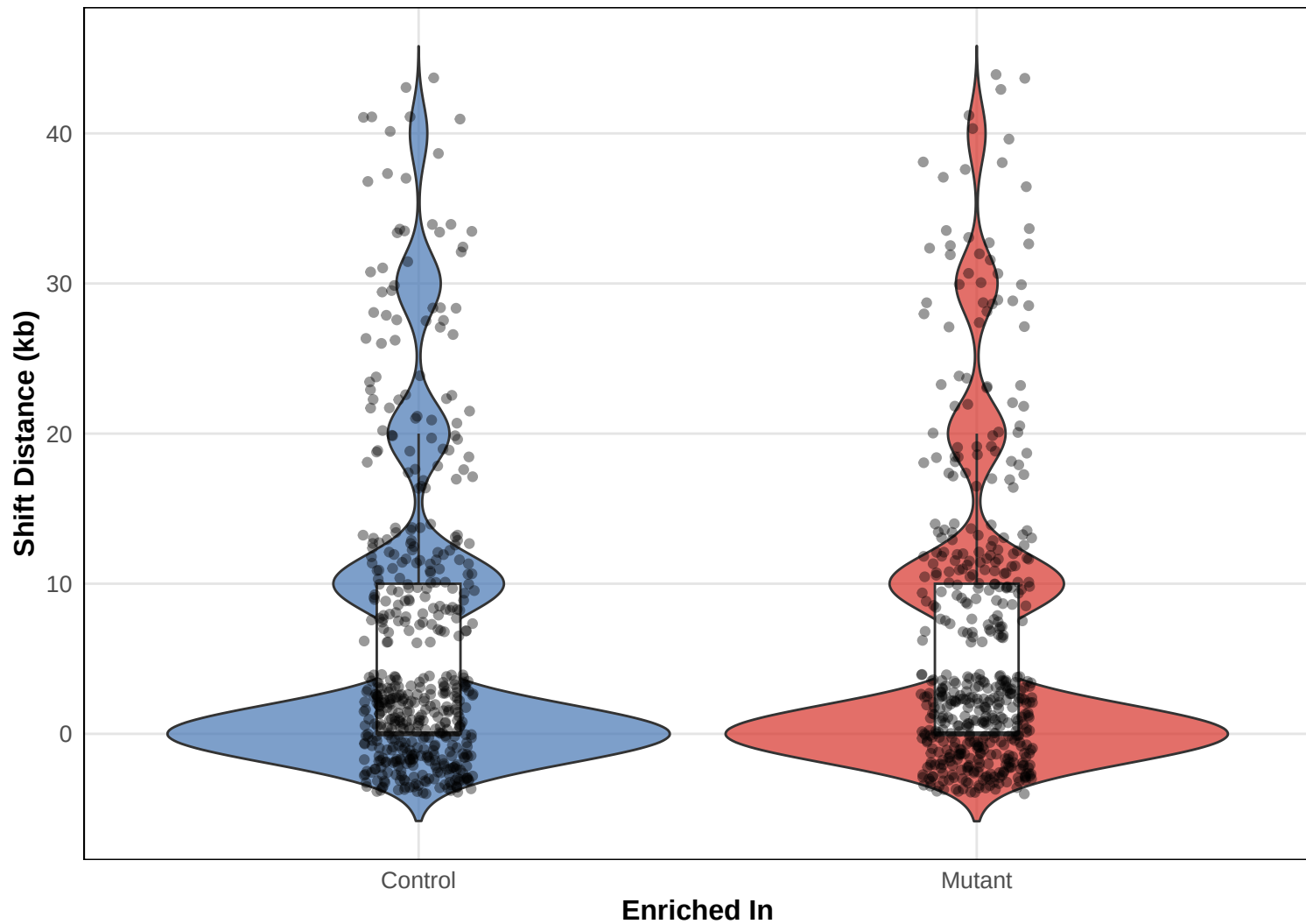
Shift Distance by Enrichment Direction
